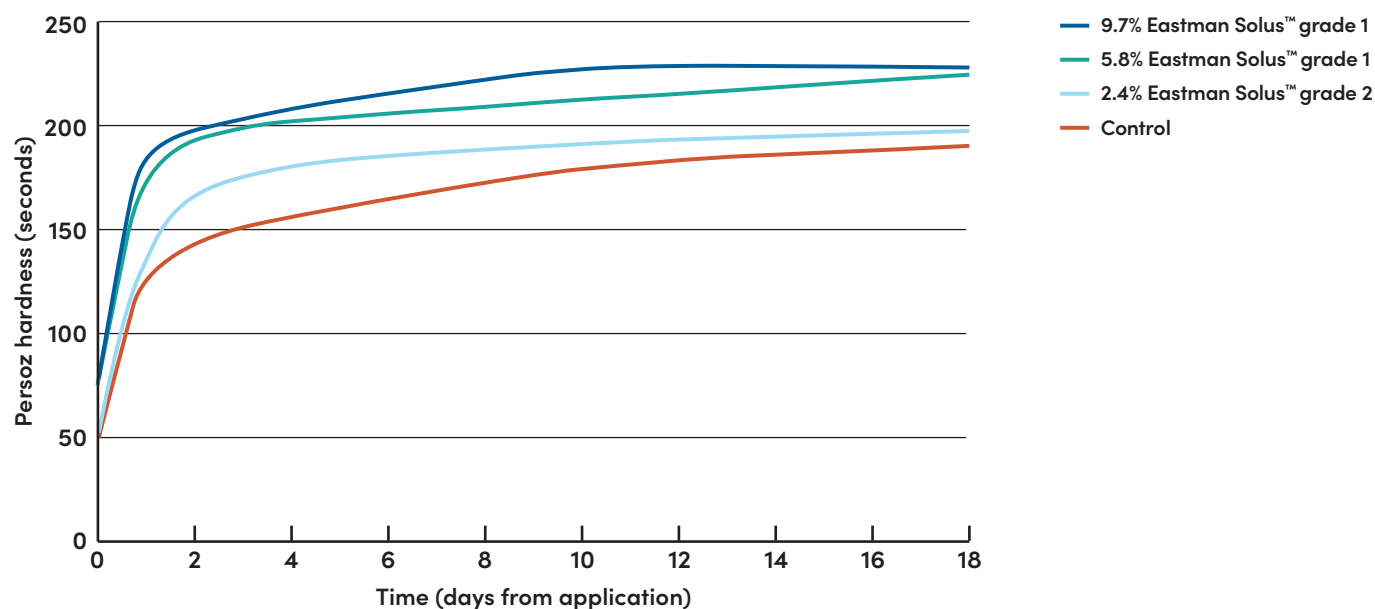
Figure 2. Persoz hardness development over 18 days
